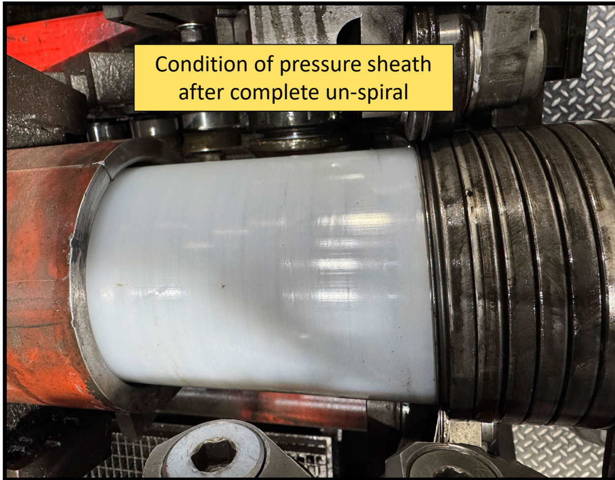
Figure 2 : Reparation by un-spiral has been performed to re-position the wires to be in a good spiral. Thus, this reparation was accepted as it is and the dimensional after the repair is within the criteria.
