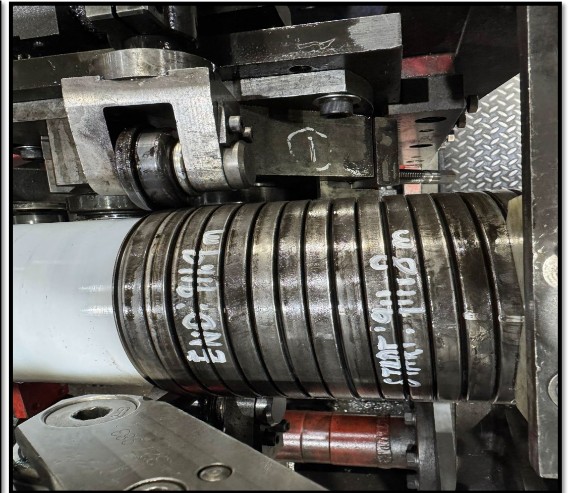
Figure 2 : Reparation by un-spiral has been performed to re-position the wires to be in a good spiral. Thus, this reparation was accepted as it is and the dimensional after the repair is within the criteria.
